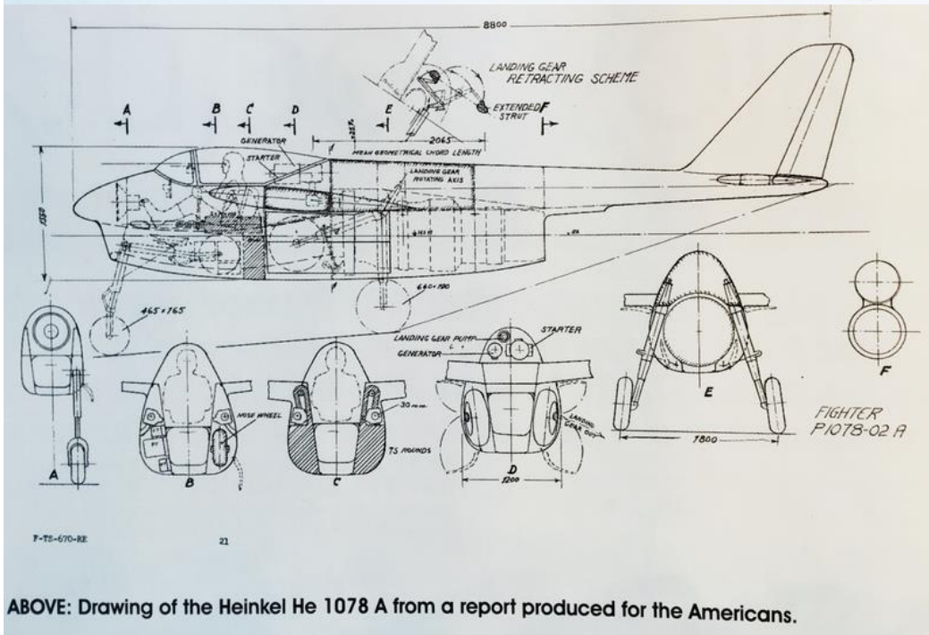
ABOVE: The He 1078 A appears to combine elements of the P 1078.01 with aspects of the He 162.
