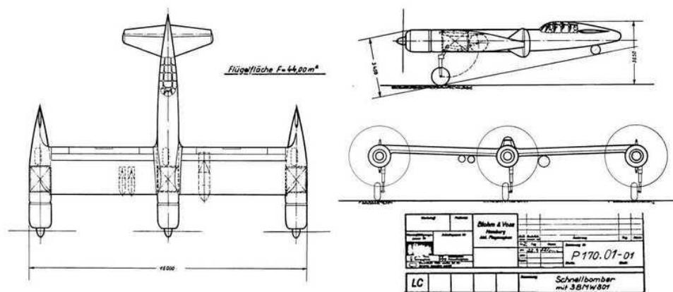
BV P170 (Propeller, bomber, 1942 Trimotor with wingtip nacelles.)
