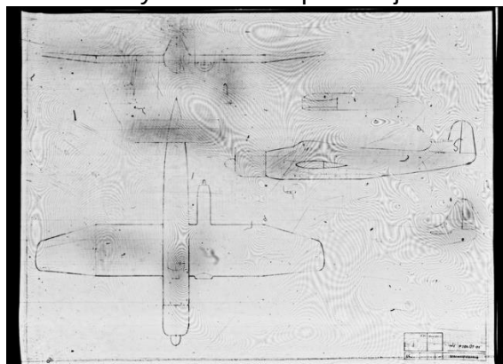
BV P204 Asymmetric. Propeller + jet.
