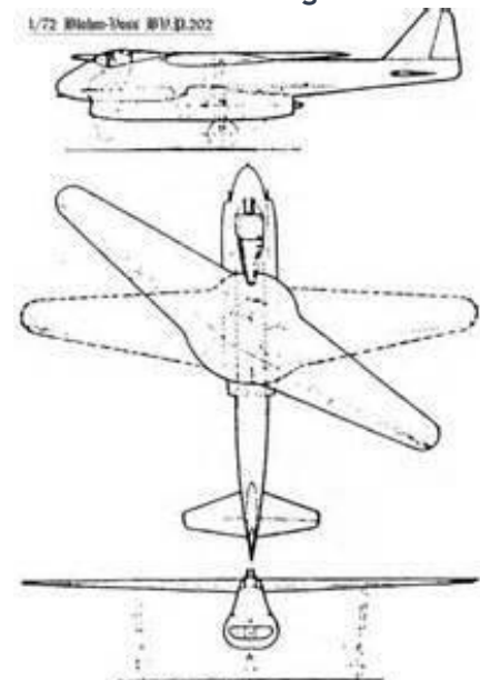
BV P202 Slewed wing
