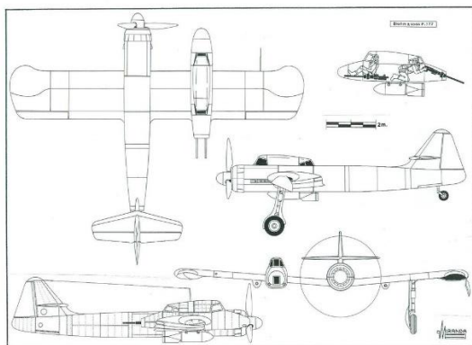
BV P177 (Asymmetric fighter/bomber)
