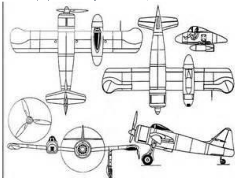
BV P179 (Asymmetric fighter/bomber)
