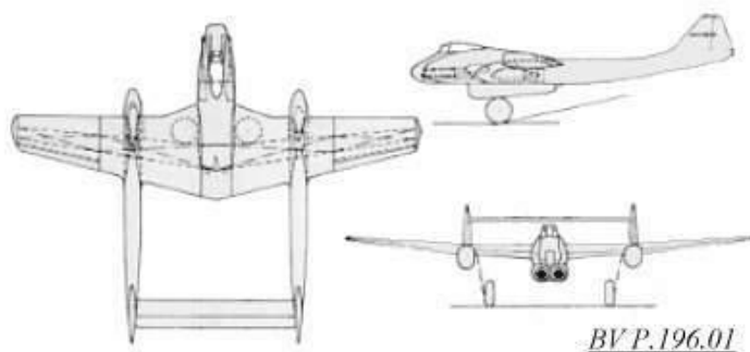
BV P196 Twin-boom.
